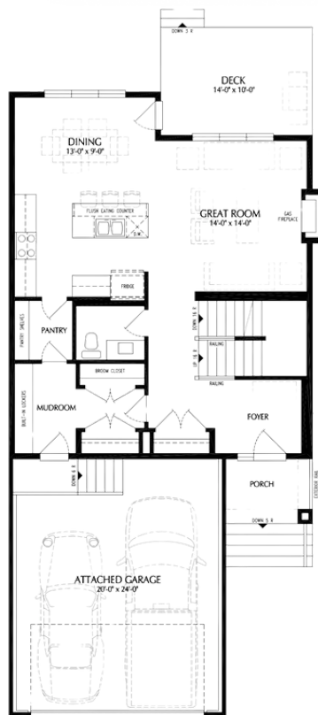
MAIN FLOOR: 895 SQ.FT.
