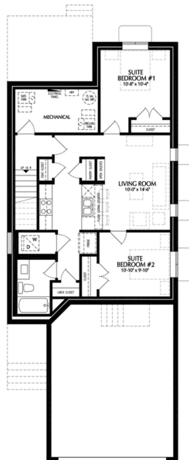
SECONDARY BASEMENT SUITE: 722 SQ.FT.
